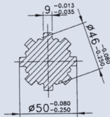
SPLINED SHAFT
