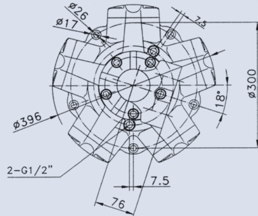
PARALLEL SHAFT (P)
