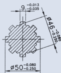
SPLINED SHAFT
