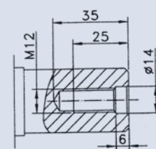
FIX HOLE (FOR ALL SHAFT)
