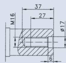
FIX HOLE (OPTION)
