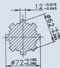
SPLINED SHAFT 62 UNI 221
