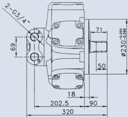
SPLINED SHAFT
