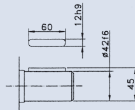
PARALLEL SHAFT (P)
