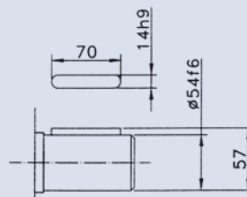
PARALLEL SHAFT (P)
