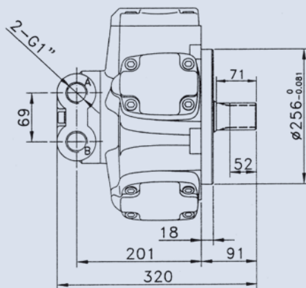
SPLINED SHAFT
