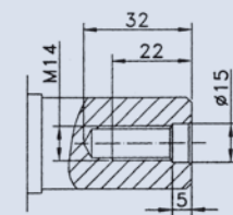
FIX HOLE (OPTION)
