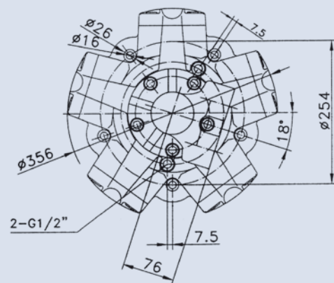
PARALLEL SHAFT (P)
