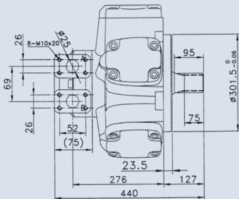
SPLINED SHAFT 62 UNI 221
