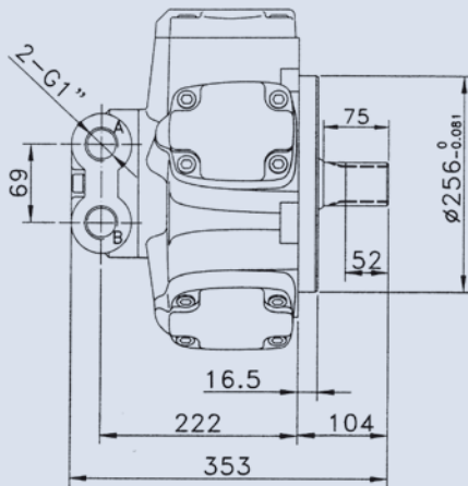
SPLINED SHAFT
