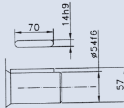
PARALLEL SHAFT (P)
