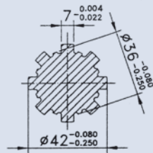
SPLINED SHAFT
